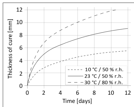
Diagram 1: Curing speed Sikaflex®-260 N
