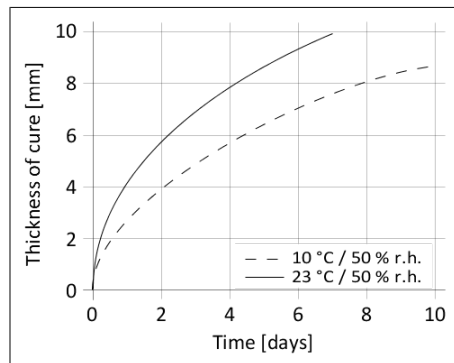
Diagram 1: Curing speed Sikaflex®-258
